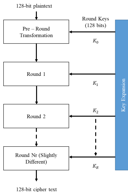
Figure 4 Process of Conventional Advanced Encryption Standard
