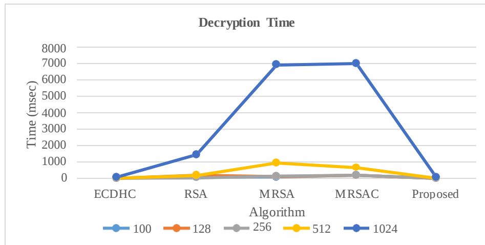
Figure 13 Comparative Analysis of decryption time for varied key lengths [45]
