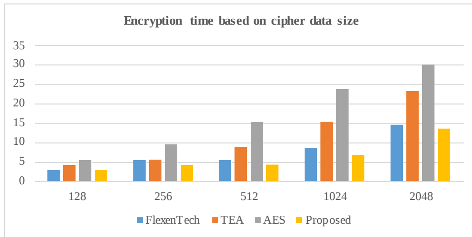
Figure 9 Analysis of encryption time for varied cipher data size (in byte) [43]
