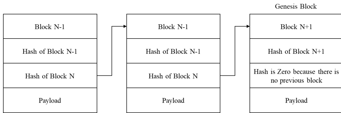
Figure 3 Blockchain hash generation (data transfer)
