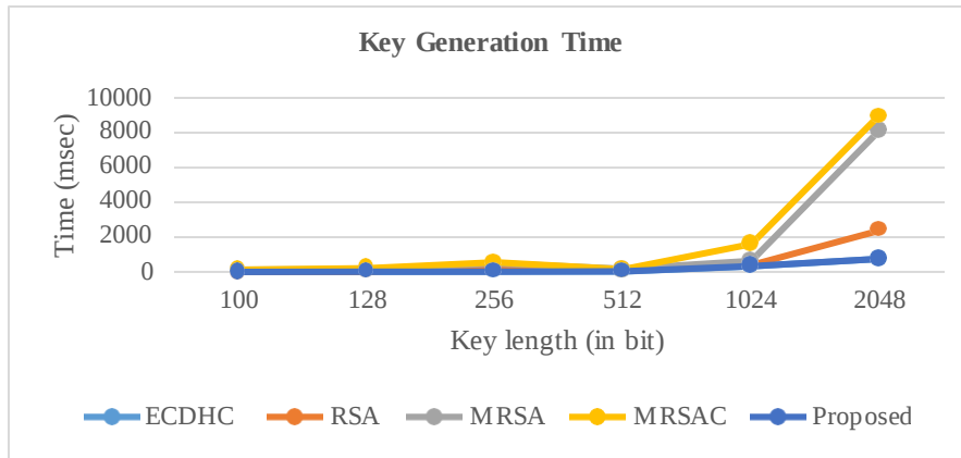
Figure 11 Comparative Analysis of key generation time for varied key length [45]
