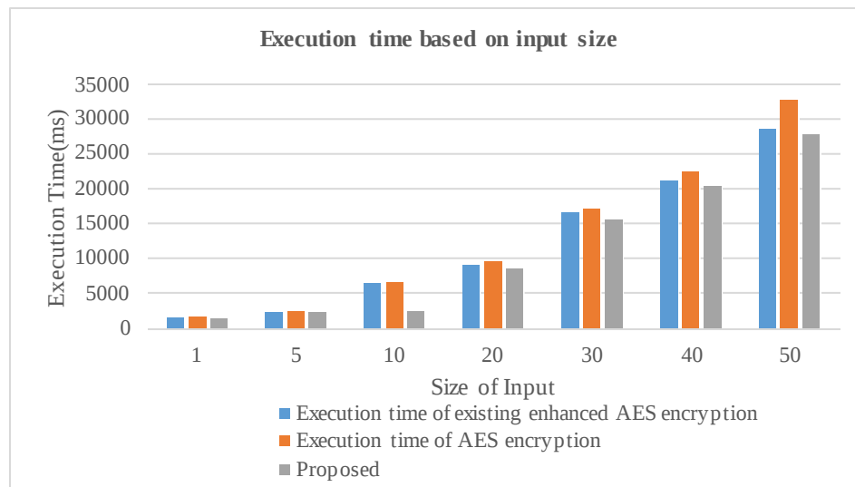
Figure 8 Analysis concerning execution time for varied input sizes [42] (in blocks, one block=128 bit)
