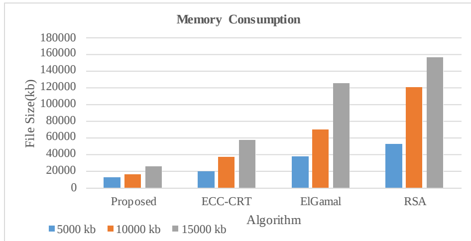
Figure 10 Analysis of memory consumption for varied file sizes [44]
