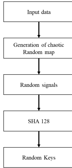
Figure 5 M-AES with Chaotic Random Key Generation
