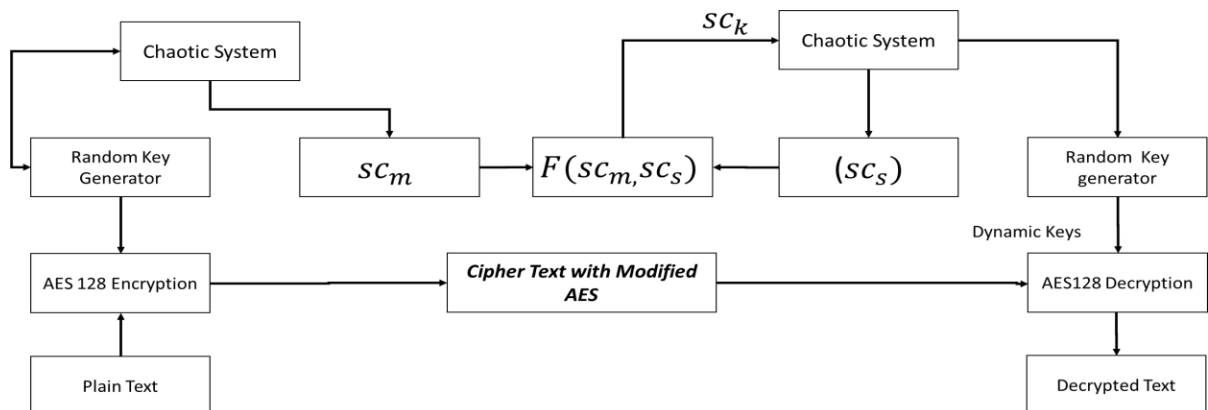
Figure 6 Process of Modified-Advanced Encryption Standard
