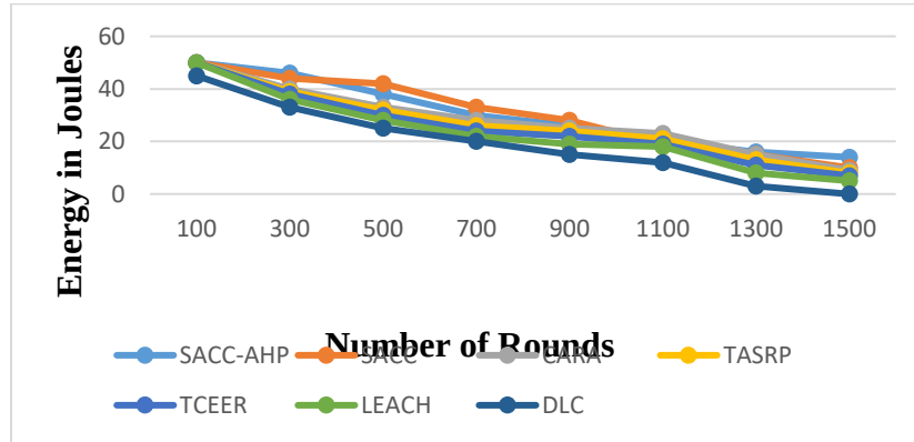
Figure 4: Energy consumption analysis
