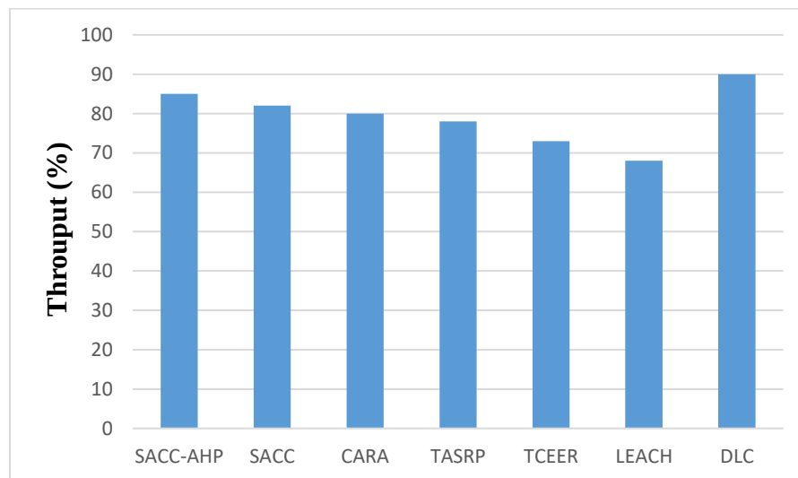
Figure 6: Throughput analysis
