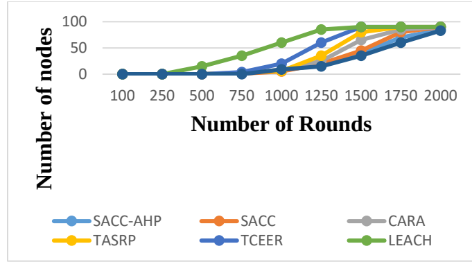
Figure 5: Network Lifetime Analysis
