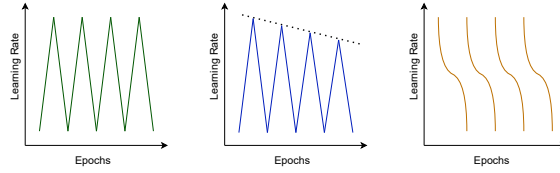
Figure 2: Examples of learning rate scheduling
