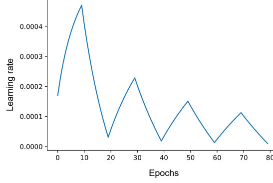
Figure 4: Example of cyclic learning rate decay
