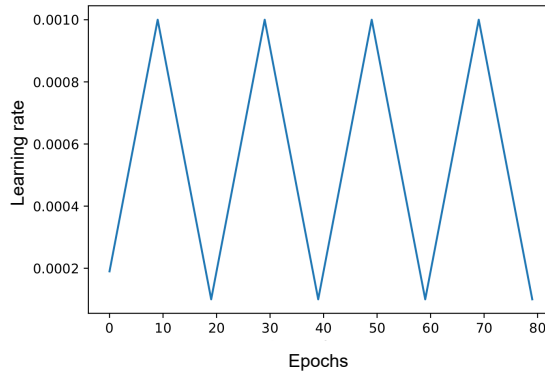
Figure 3: Example of cyclic learning rate
